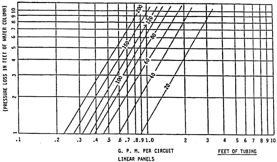
Linear Panel Pressure Drop Curve
